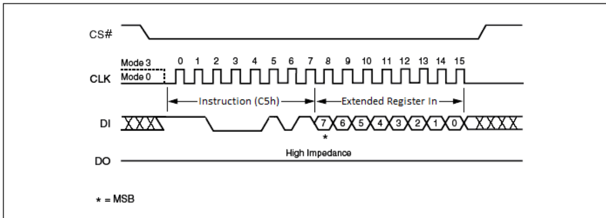
Write Extended Register Instruction Sequence Diagram
