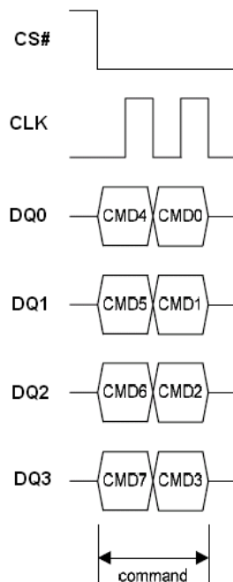
Chip Erase Instruction Sequence Diagram
