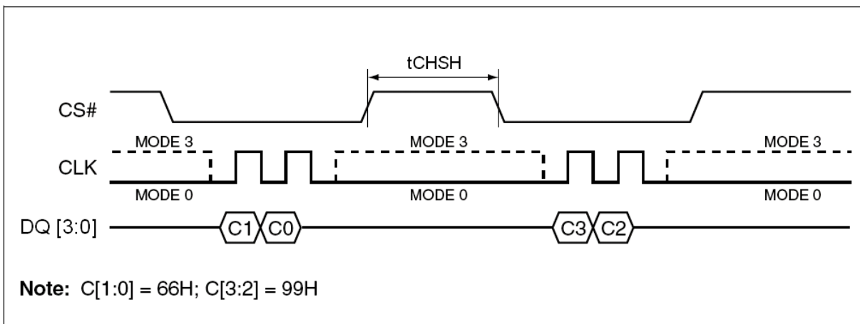
Reset-Enable and Reset Sequence Diagram under QPI Mode
